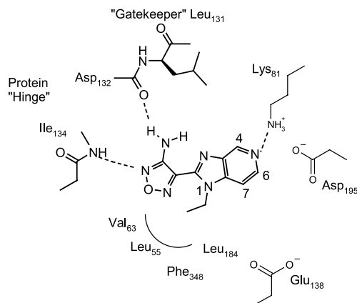
Figure 1. GOLD docking of compound 2 into an MSK-1 homology model.
