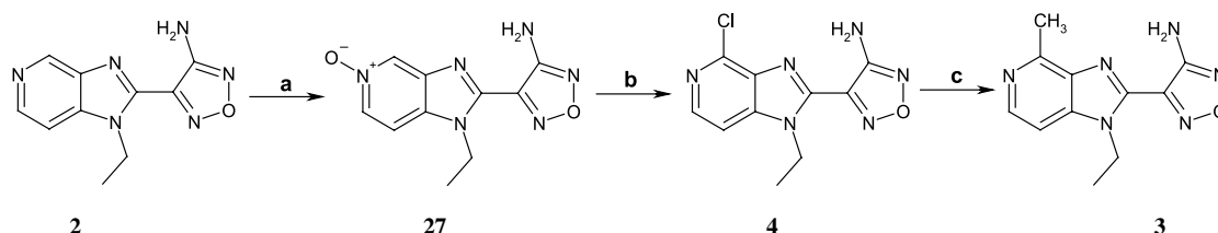
Scheme 1. Preparation of 4-substituted aza-benzimidazole derivatives 3 and 4 . Reagents and conditions: (a) 30% H 2 O 2 , AcOH, 90 °C (53%); (b) POCl 3 , 120 °C (100%); (c) 2 M Al(CH 3 ) 3 in toluene, 1,4-dioxan, Pd(PPh 3 ) 2 Cl 2 , reflux (13%).
