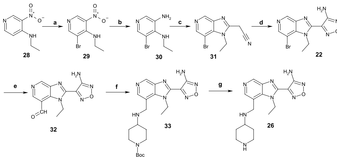
Scheme 2. Preparation of 7-substituted aza-benzimidazole derivatives 22 and 26 . Reagents and conditions: (a) Br 2 , AcOH, 100 °C (43%); (b) sodium dithionite, ethanol/water, 60 °C; (c) Ethyl cyanoacetate, 190 °C (35%, two steps); (d) (i) NaNO 2 , MeOH, HCl, rt; (ii) NH 2 OH, NaOH, reflux (45%, 2 steps); (e) n -BuLi, DMF, THF, −78 °C (41%); (f) 4-amino-piperidine-1-carboxylic acid tert -butyl ester, (polystyrylmethyl)trimethylammonium cyanoborohydride, MeOH, AcOH, 21 °C (42%); (g) TFA, DCM, 21 °C (82%).
